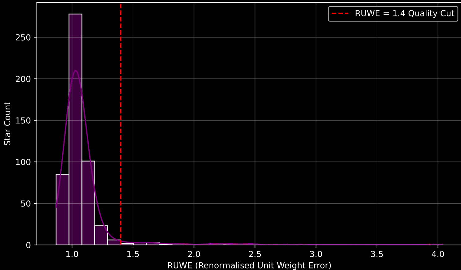
GAPOGEE DR17 Field [210+00] RUWE Distribution (n= 512)
