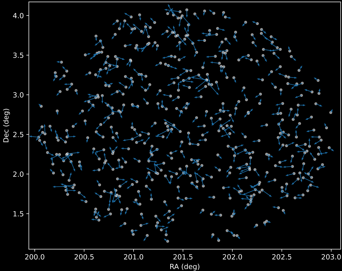
APOGEE DR17 Cluster 0 Proper Motion Vectors (n=475)
