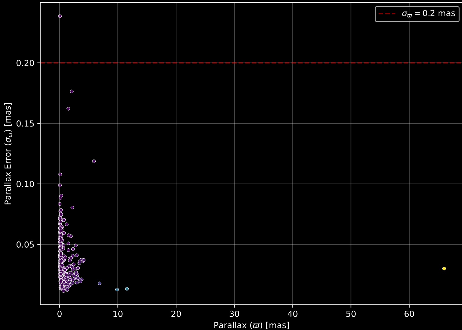
APOGEE DR17 Field: [210+00] Parallax Quality (n= 514)
