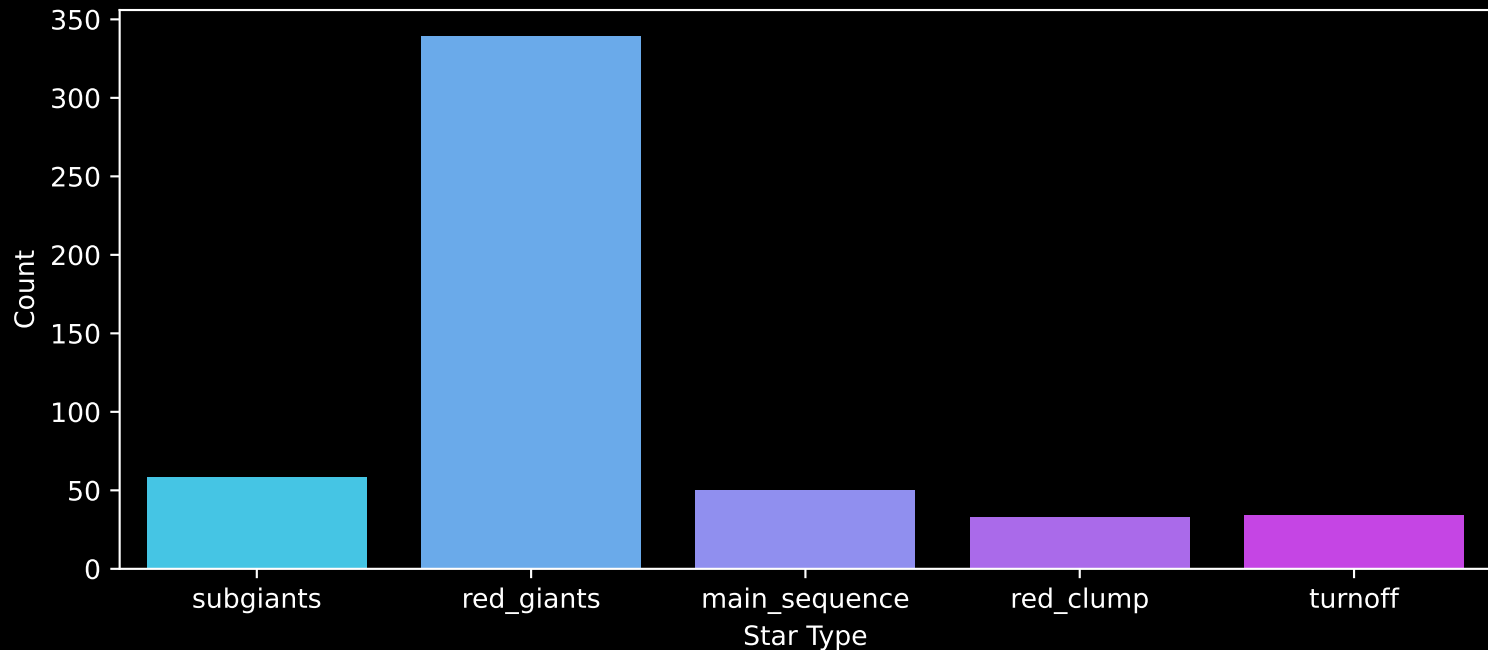
APOGEE DR17 Field: [210+00] Count plot of Star Type
