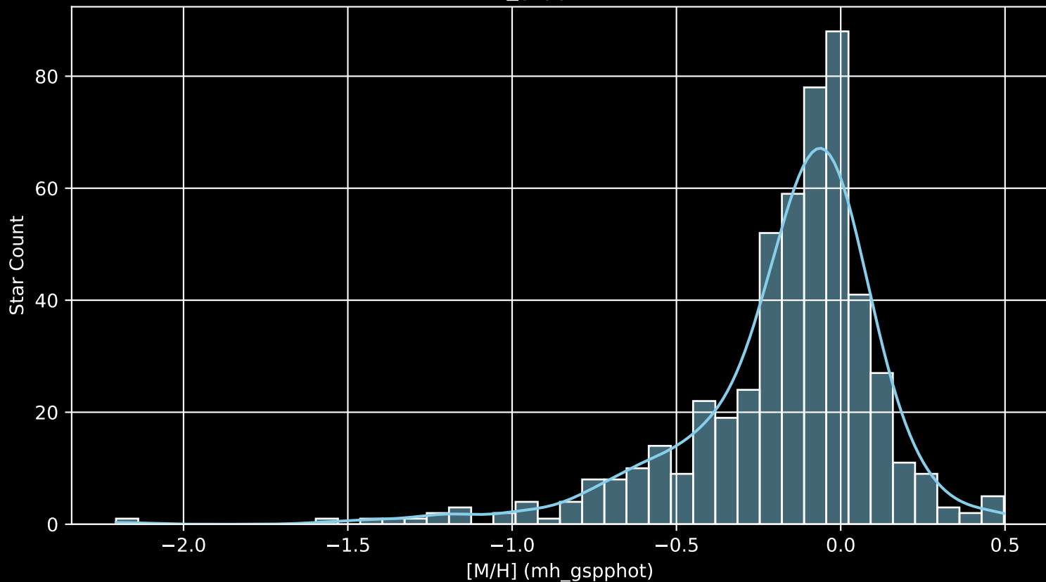
APOGEE DR17 Field: [210+00 [M/H] (mh_gspphot) (n= 510)
