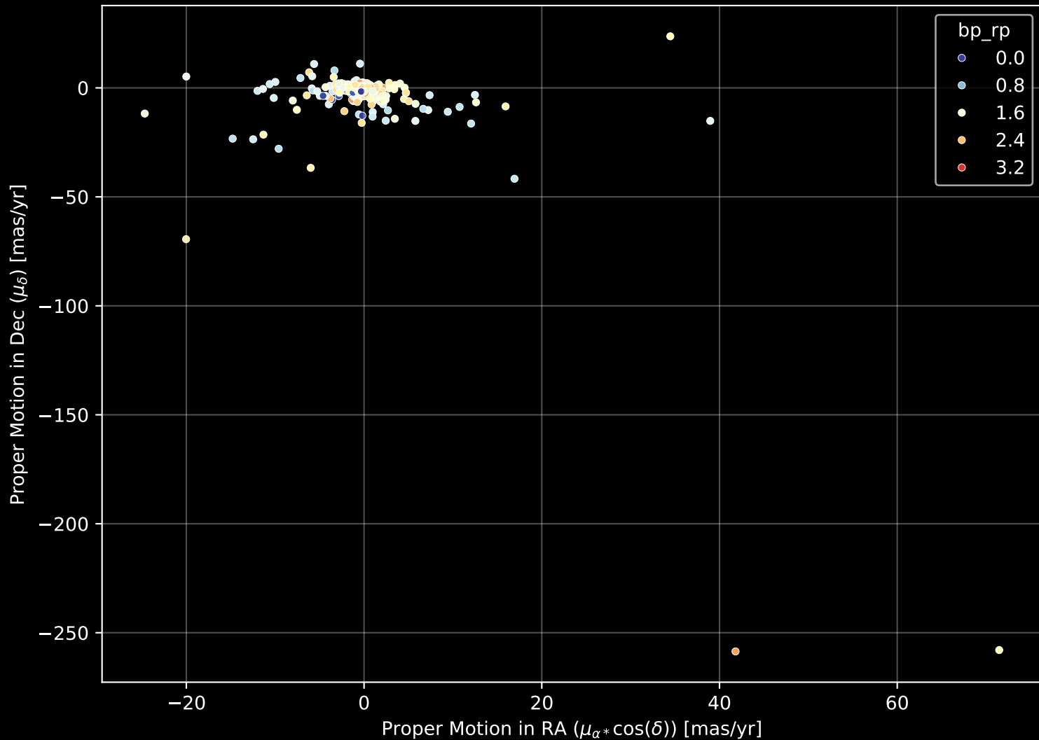
APOGEE DR17 Field: [210+00] Proper Motion Diagram (n= 514)
