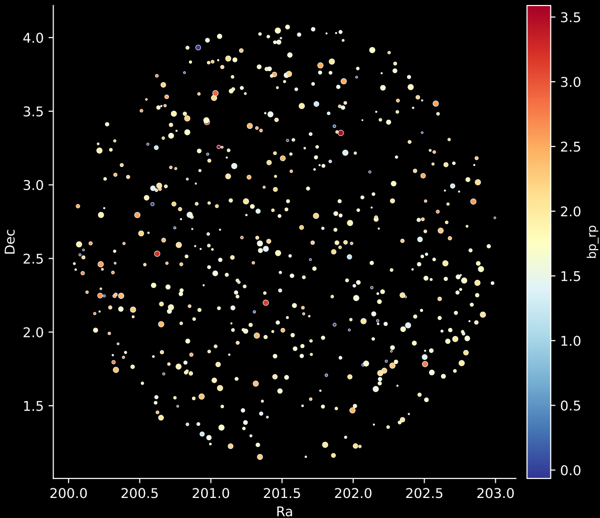
APOGEE DR17 Field: [210+00] Stars: 514
